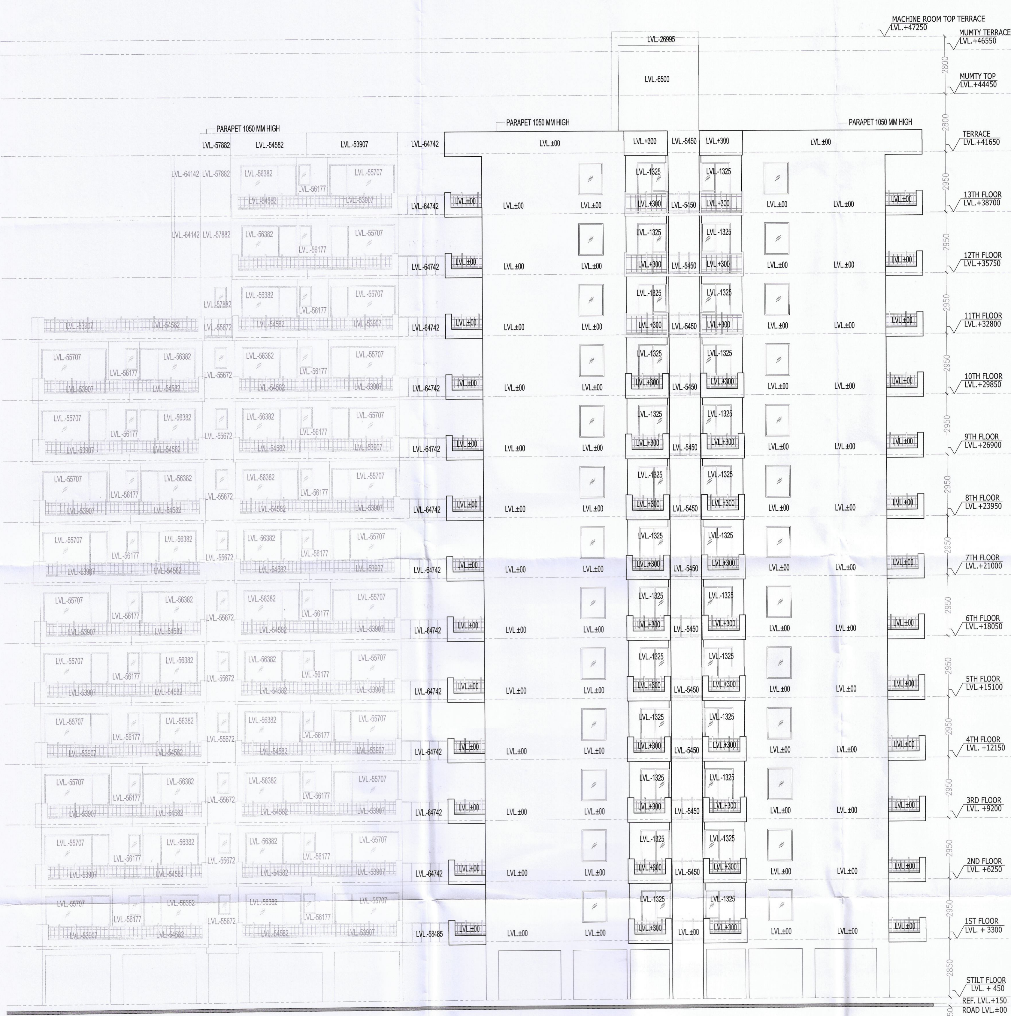
TOWER-2 ELEVATION -4
