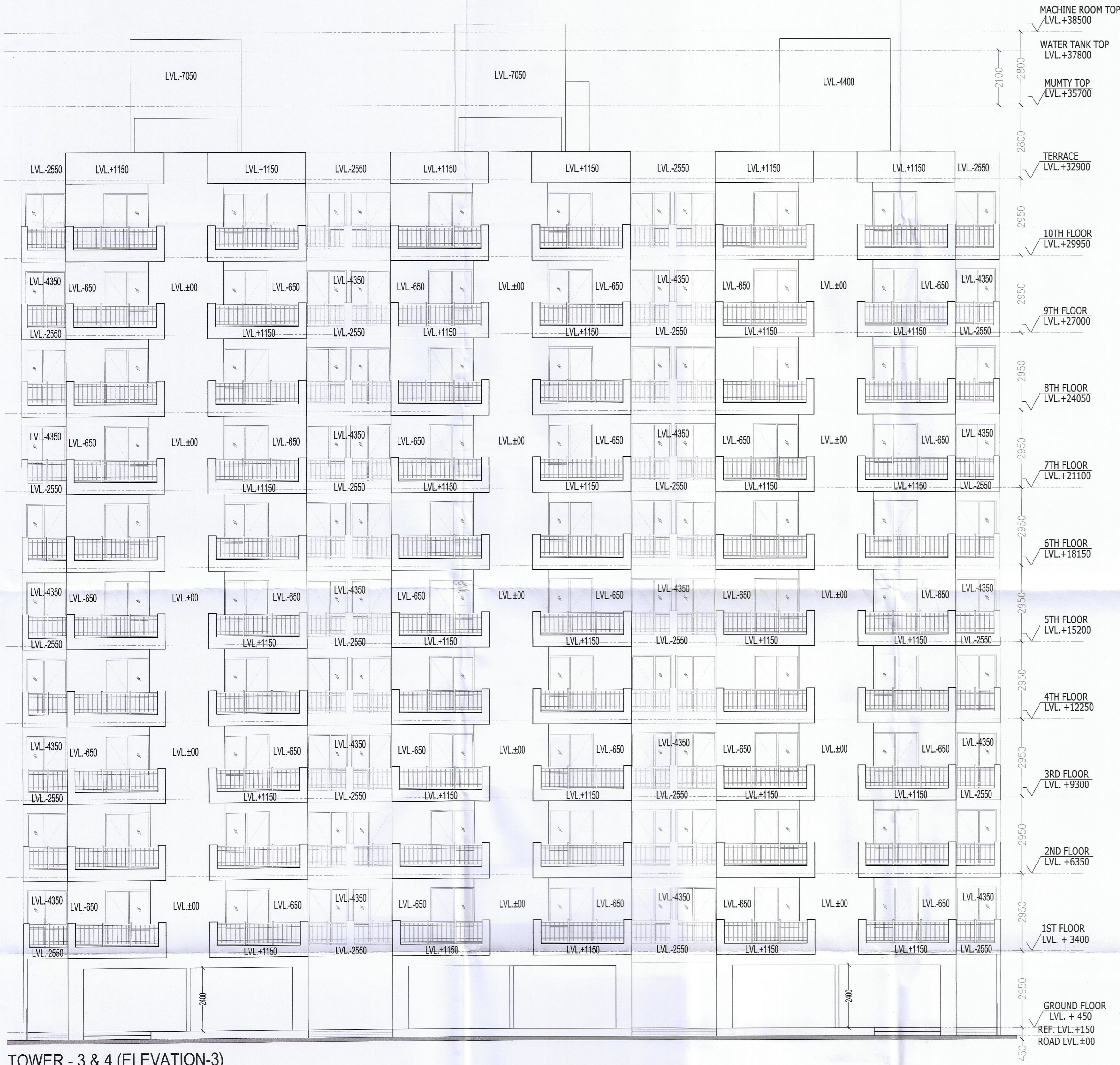
TOWER - 3 & 4 (ELEVATION-3)
