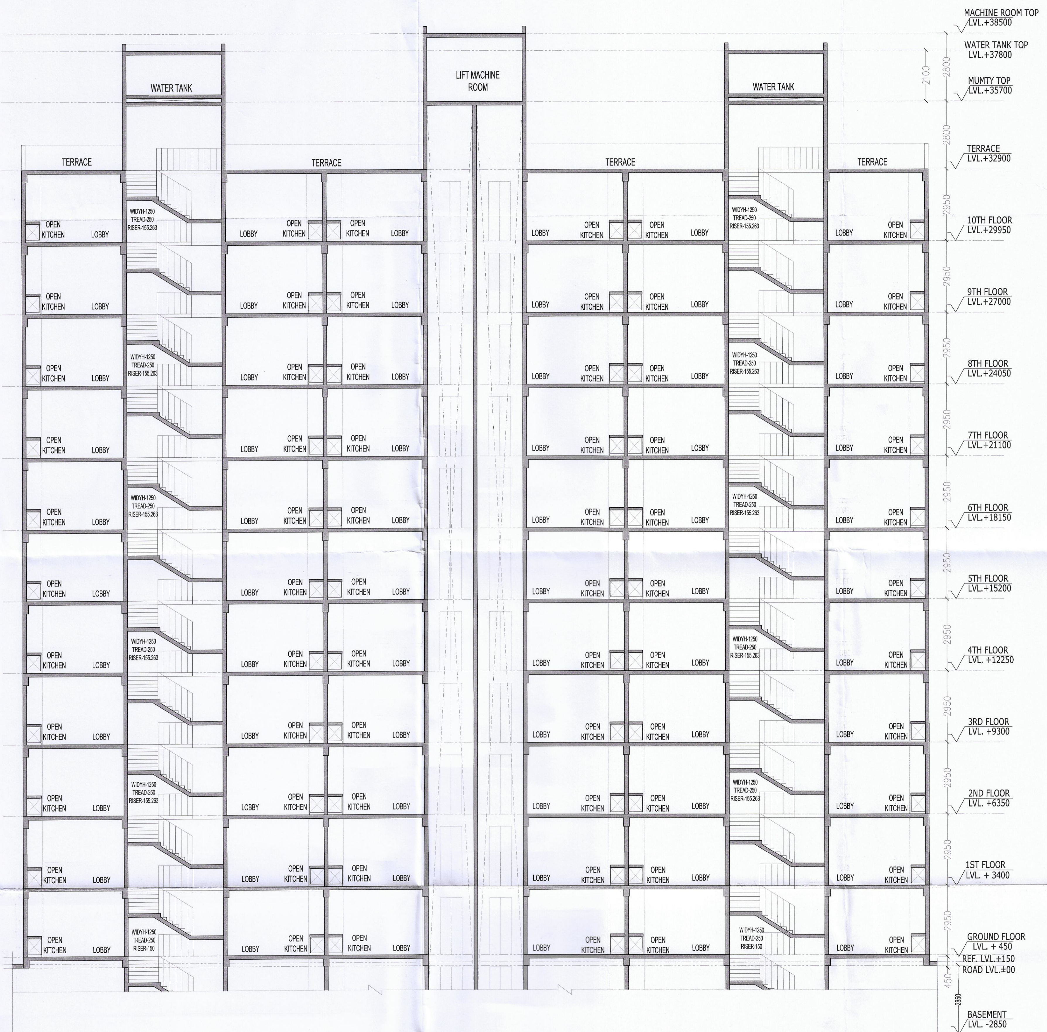
TOWER-3 & 4 (SECTION- Y,Y)
