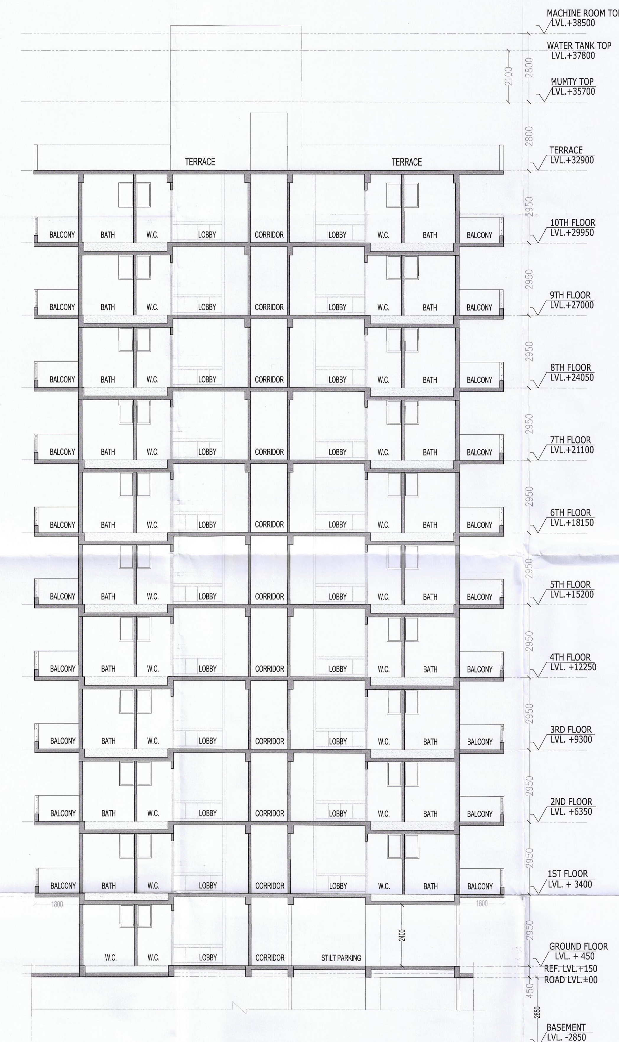
TOWER-3 & 4 (SECTION- X,X)
